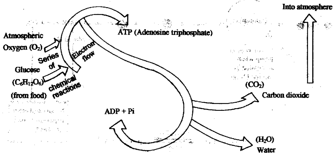
Fig. 32.1 Cellular Respiration
