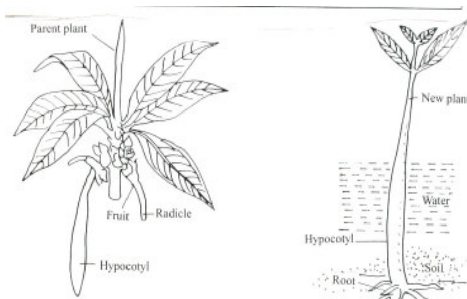
Fig 19.5 Vivipary Germination
