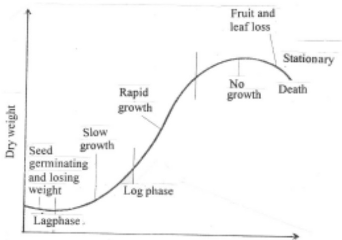
Fig. 19.2 Sigmoid curve
